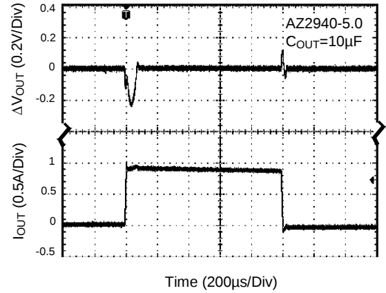
Load Transient
