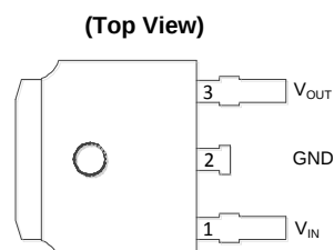
TO-252-2 (3) (Option 2)
