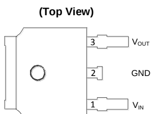
TO-252-2 (3) (Option 1)
